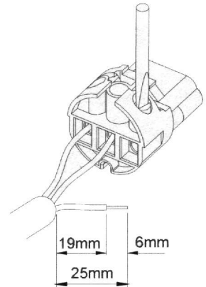
Fig.3 Cutting Length
