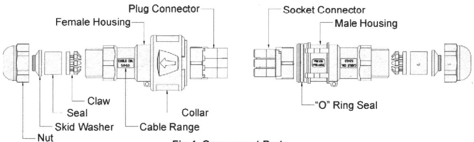
Fig.4 Component Parts
