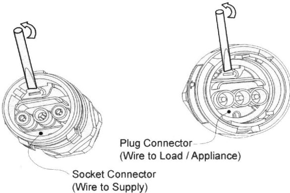
Fig.2 Inner Connectors
